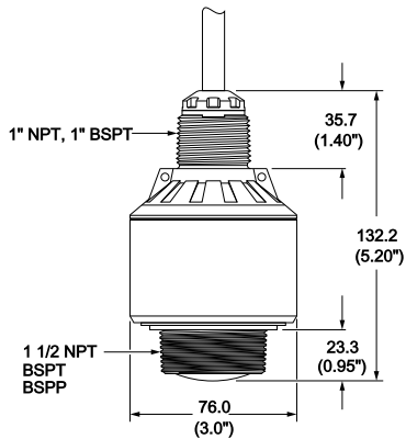
Figure 12.4 Encombrement SITRANS LR100
